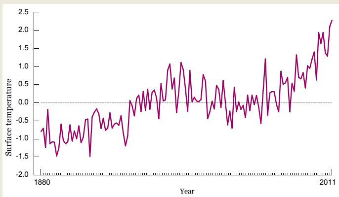
Figure 52: Surface temperature trends in the Arctic
