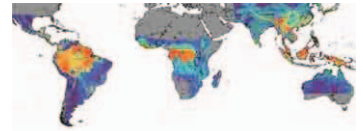
Figure 46: Regional patterns of forest above-ground biomass in tropical forests
