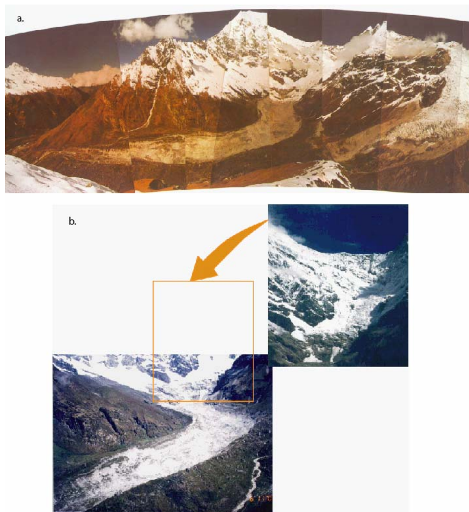
Figure12: Lirung Glacier in a. 1985 and b. 2002
