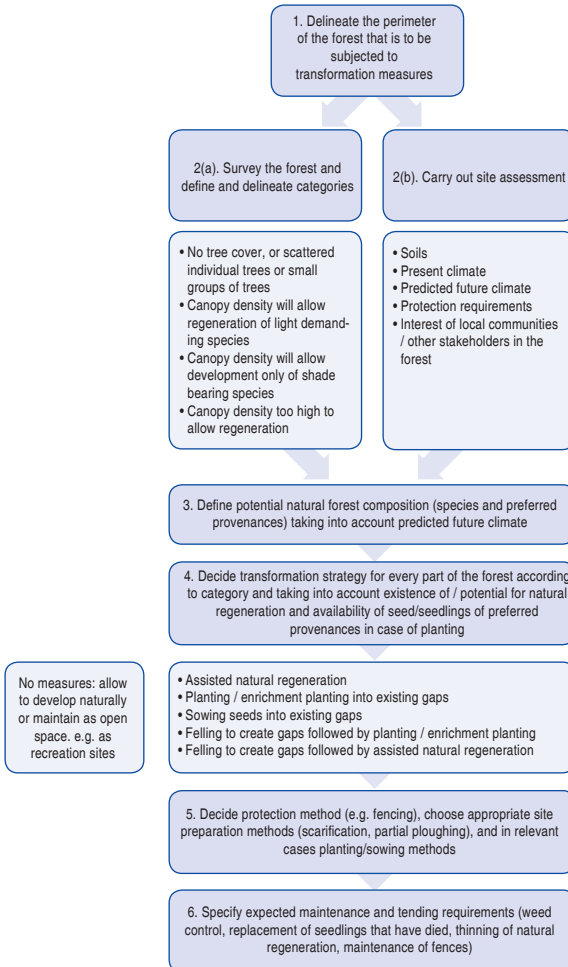
Figure 1 – Recommended process for deciding measures for transforming artificially propagated pine stands into close to nature forest stands
